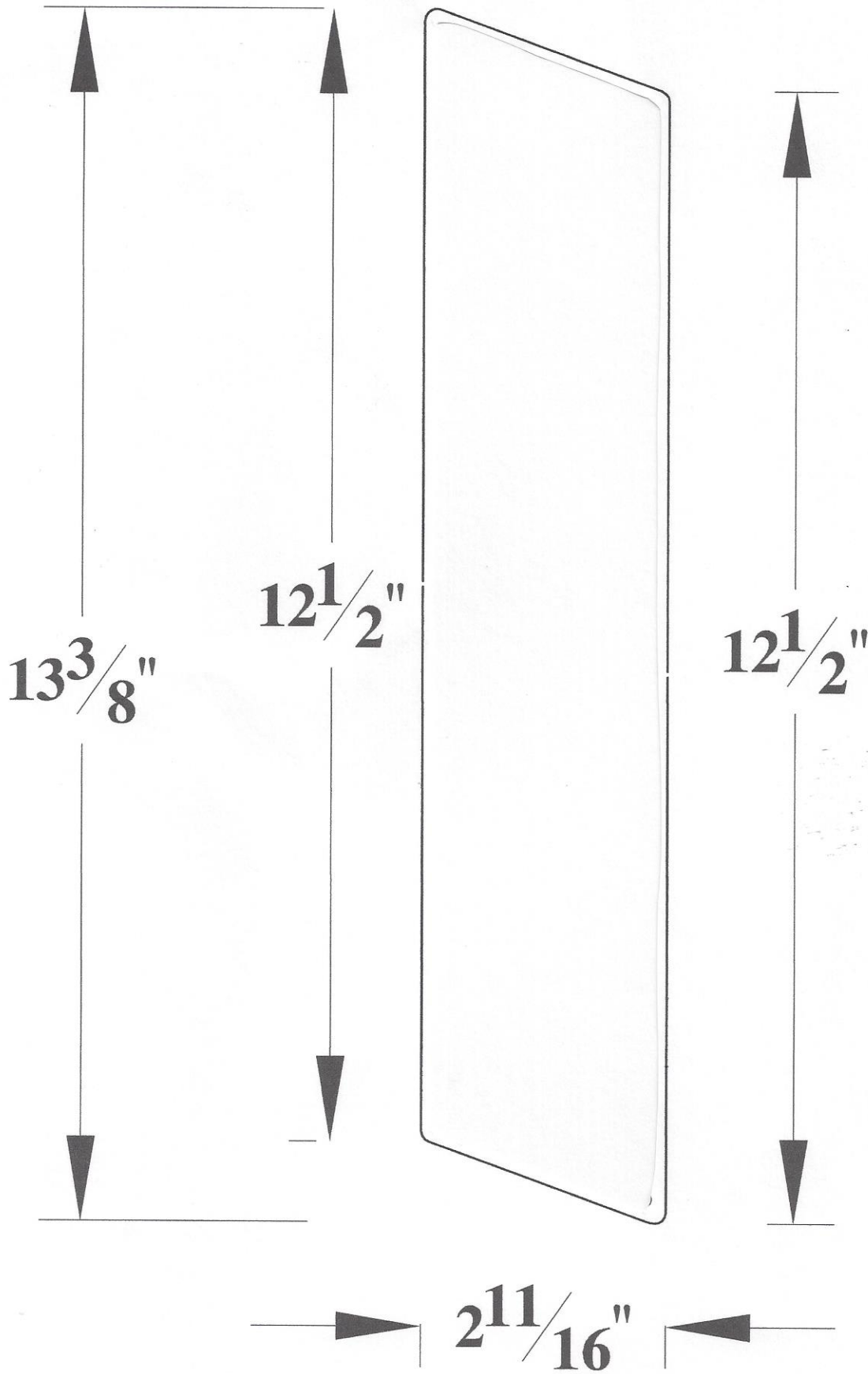
Side Louvers
