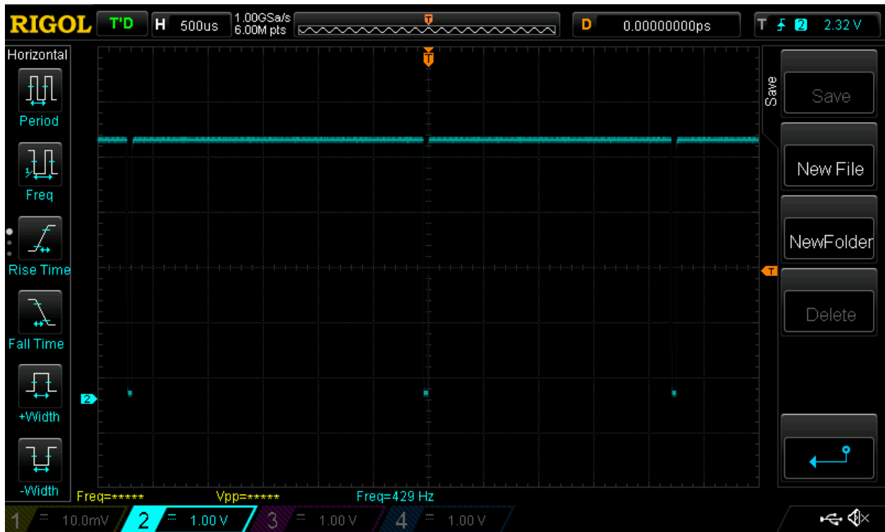
Tachometer Output of Fan operating at slowest speed.
